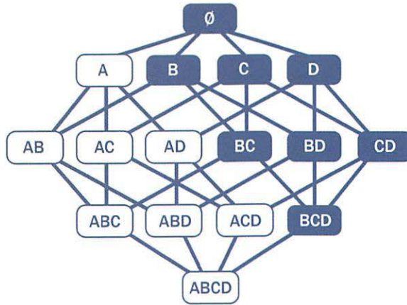
FIGURE 5-2 Itemset \{A, B, C, D\} and its subsets
