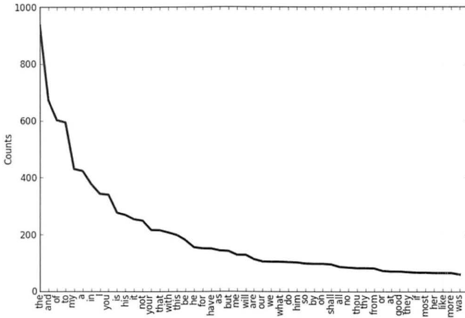
FIGURE 9-2 The 50 most frequent words in Shakespeare's Hamlet
